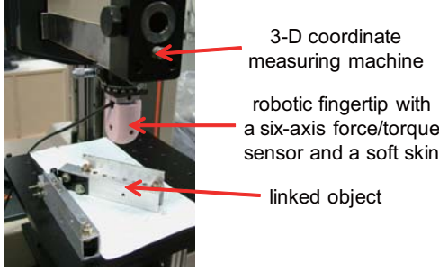
Fig. 7. Experimental setup.
