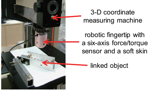
Fig. 7. Experimental setup.
