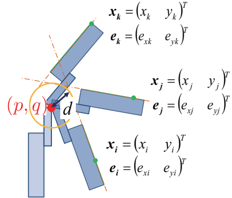
Fig. 10. Proposed method: Estimation method of the position of the joint-axis ( p , q ) based on measurement of the locations of contact points ( \mathbf{x}_i , \mathbf{x}_j , \mathbf{x}_k ) and the directions of edges of an object ( \mathbf{e}_i , \mathbf{e}_j , \mathbf{e}_k ).
