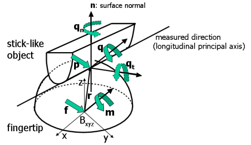
Fig. 6. Geometric relationship for soft line contact.
