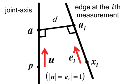
Fig. 4. Defined vectors to calculate the position and orientation of the joint-axis: \mathbf{x}_i is the position vector of the contact point at the i th measurement, \mathbf{e}_i is the direction vector of the edge of the object at the i th measurement, \mathbf{p}_i is the position vector of a point on the joint-axis, \mathbf{u} is the orientation of the joint-axis, and d = |\mathbf{a}_i - \mathbf{a}| is the distance between the edge and the joint-axis.
